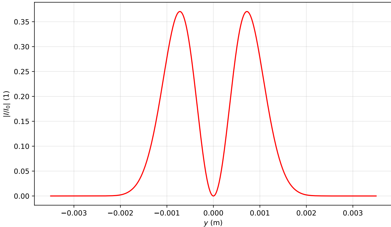
Intensity profile I(x=0, y, z=2.149)/I_0 , P_{in}=0.5P_{cr} , artificial time
